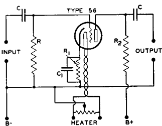
RESISTANCE-COUPLED A-F AMPLIFIER
